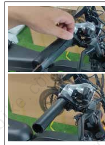
21. Remove the handle sleeve on the right
